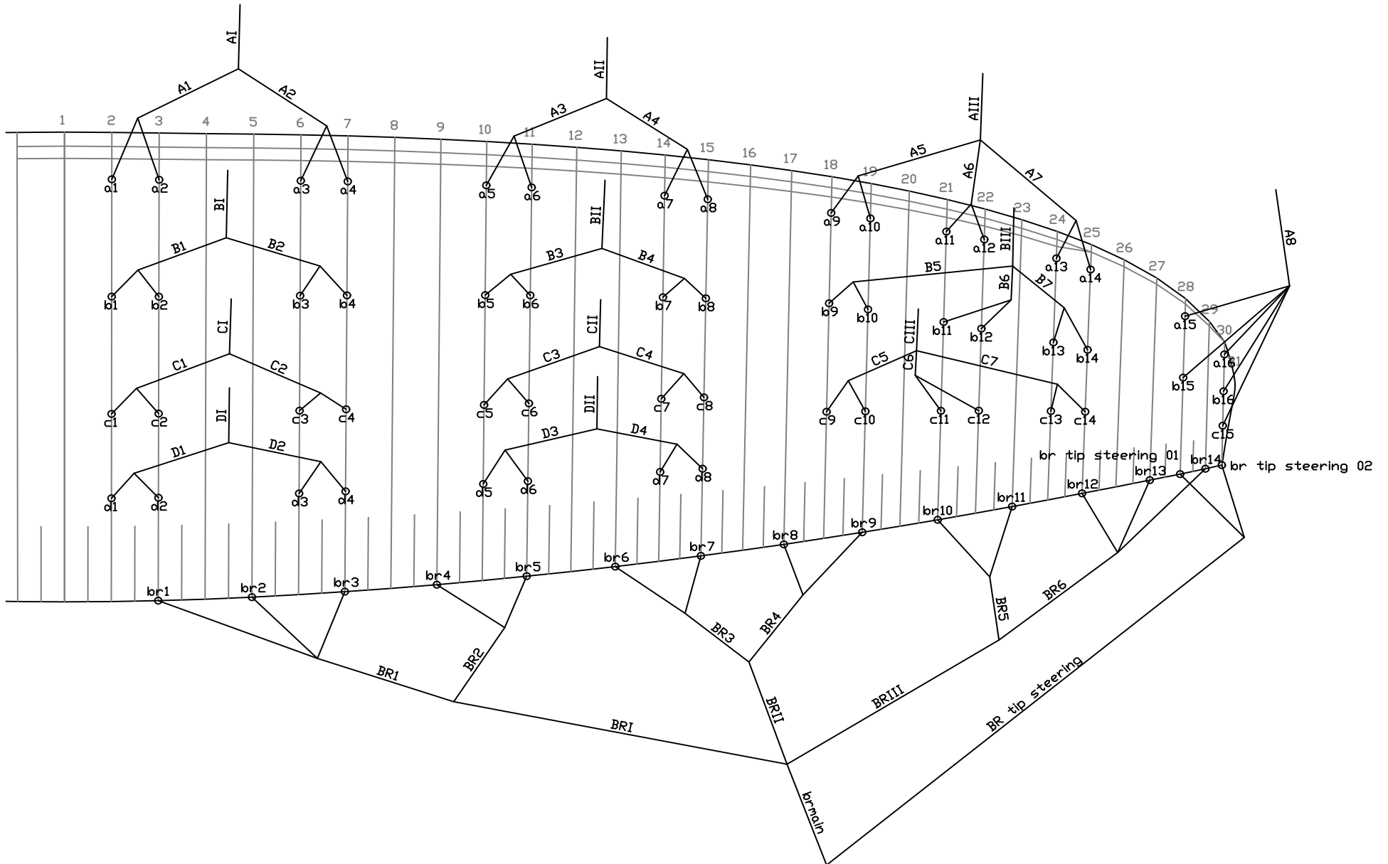
Line Plan
